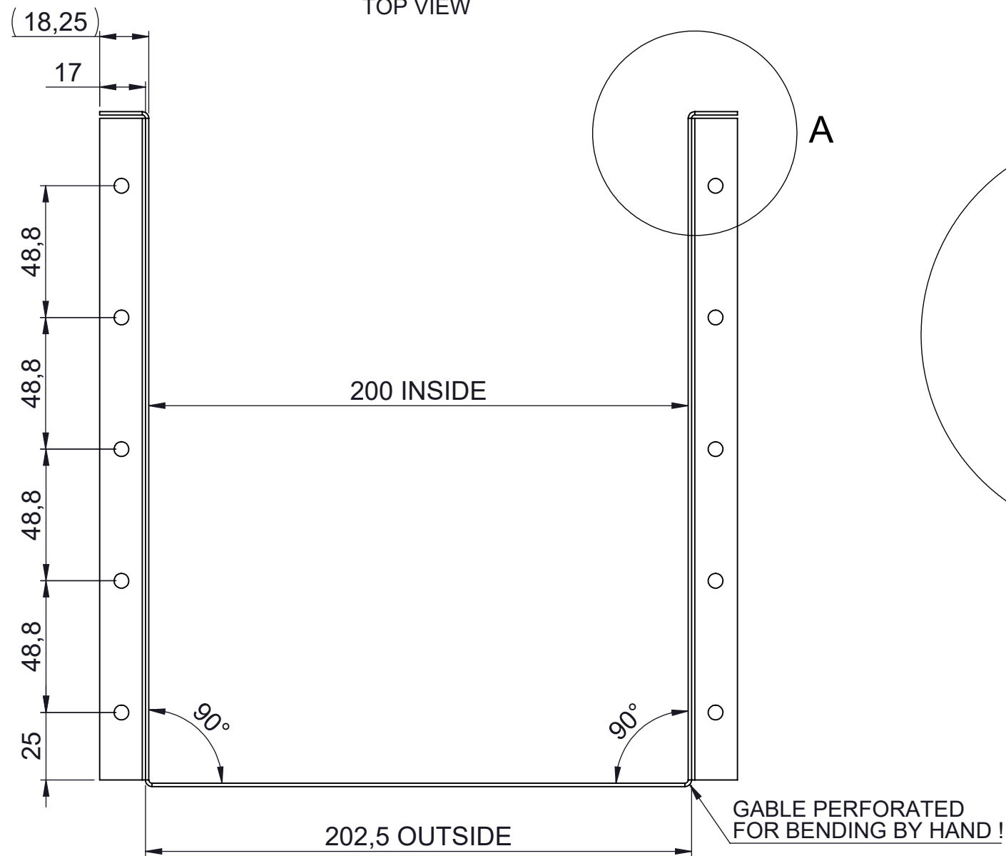
TOP VIEW
