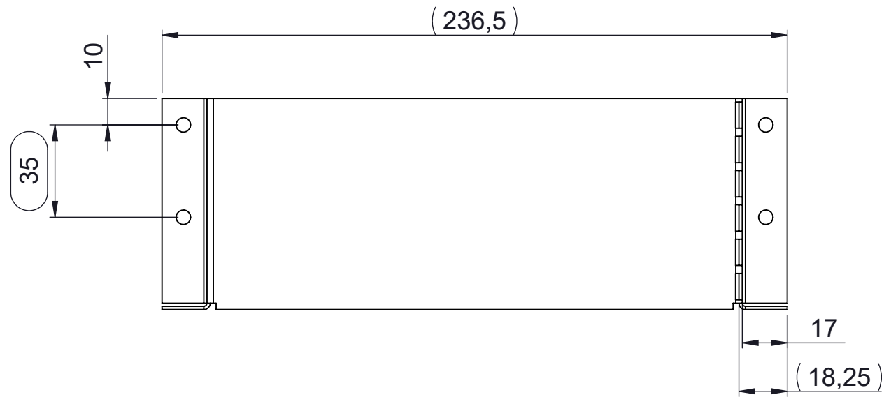
TOP VIEW
